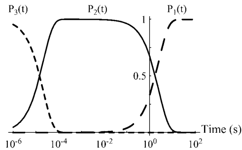
FIGURE 8 Filling up of the energy landscape wells. Probability for a bond that is initially in the outermost minimum (minimum number 3 in Fig. 4) to be in a well as a function of time. For each well, there is a sharp transition from fully occupied to empty and from empty to fully occupied at times that are orders-of-magnitude different. These curves are obtained through the master equations, Eqs. 6a–c.
